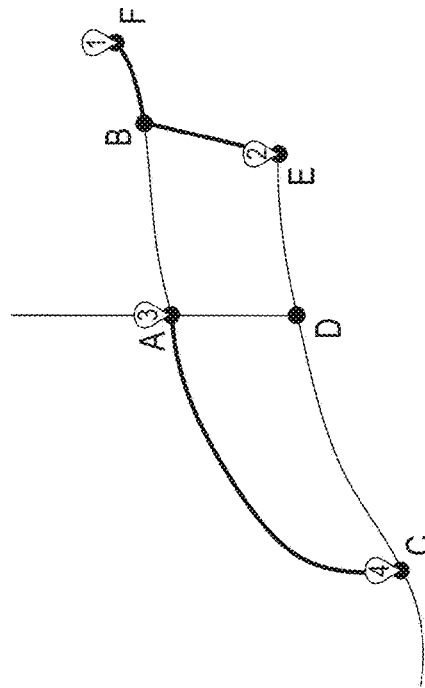
Potential Assignment 1: 1, 2 AND 3, 4
