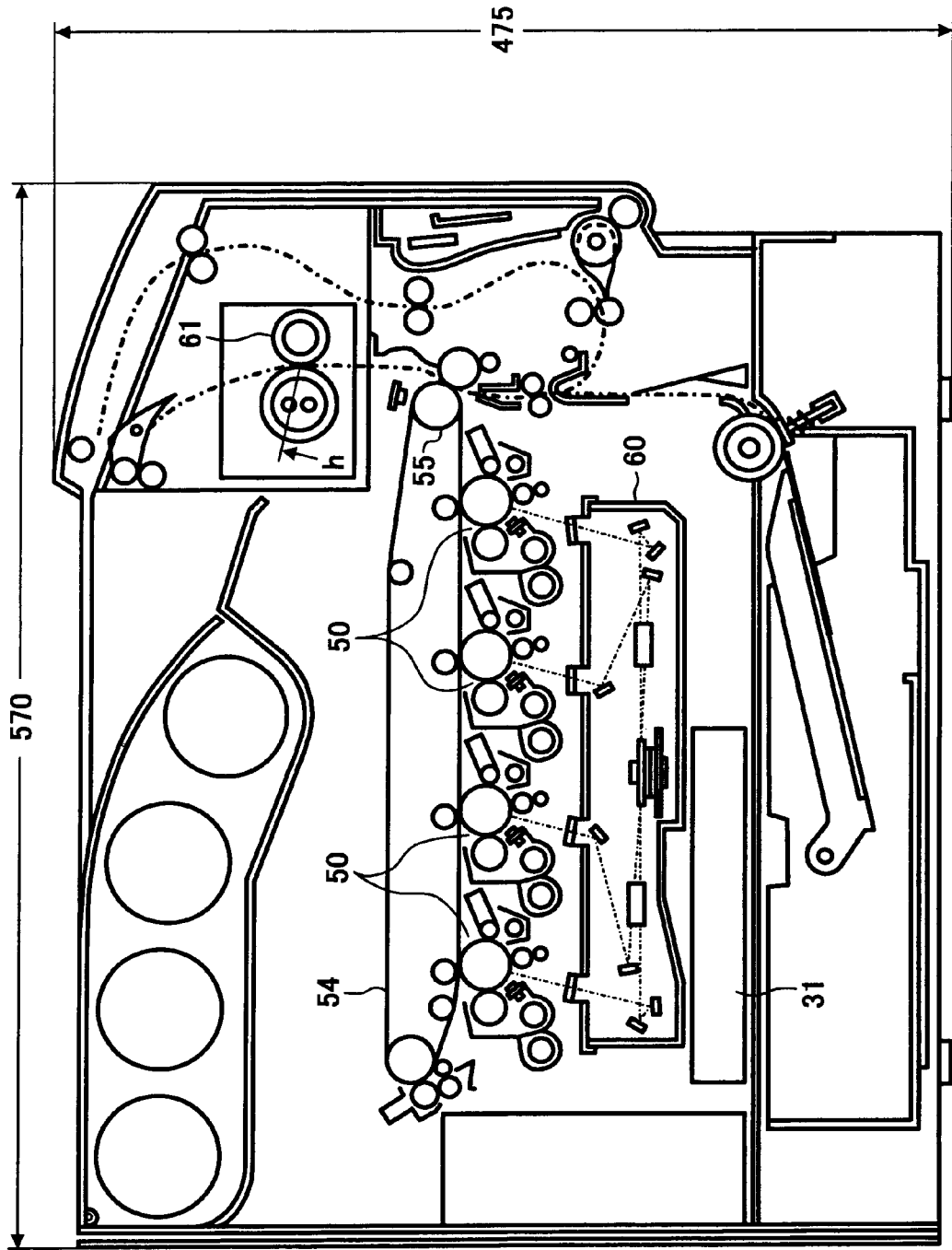
FIG. 4 PRIOR ART
