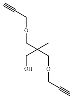
1,3-O-bis-propargyl-2-hydroxymethyl-2-methyl-1,3-propanediol (22)
