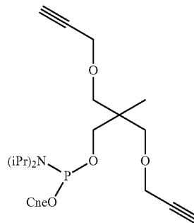
1,3-O-bis-propargyl-2-[(2-cyanoethyl)-N,N-diisopropyl-phosphoramidite]oxymethyl]-2-methyl-1,3-propanediol (23)
