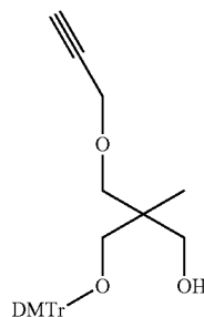
1-O-(4,4'-dimethoxytrityl)-2-propargyloxymethyl-2-methyl-1,3-propanediol (17)
