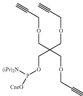
O-tris-propargyl-O-[(2-cyanoethyl)-N,N-diisopropyl-phosphoramidite]-pentaerythritol. (14)
