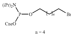
O-[(2-cyanoethyl)-N,N-diisopropyl-phosphoramidite] 6-bromo-hexan-1-ol (31)
