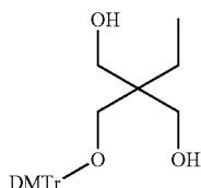
1-O-(4,4'-dimethoxytrityl)-2-hydroxymethyl-2-methyl-1,3-propanediol (16)
