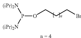
6-bromo-hexan-1-ol tetraisopropylphosphorodiamidite (32)
