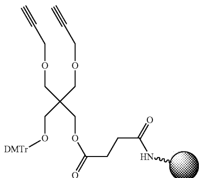
1-O-(4,4'-dimethoxytrityloxymethyl)-2,2-bis-propargyloxymethyl-3-O-(succinic-LCAA CPG)-1,3-propanediol (11)
