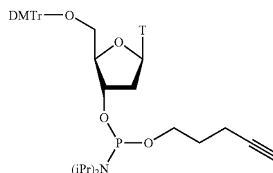
5'-O-Dimethoxytrityl-3'-O-[(4-propynyl)-N,N-diisopropyl-phosphoramidite] Thymidine (28)
