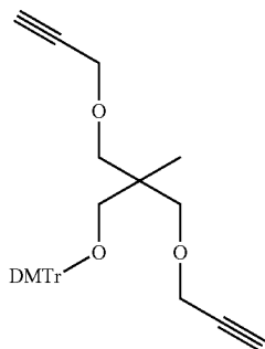
1,3-O-bis-propargyl-2-[O-(4,4'-dimethoxytrityloxymethyl)oxymethyl]-2-methyl-1,3-propanediol (21)
