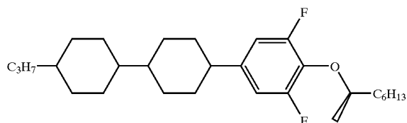
(Chemical 3)
