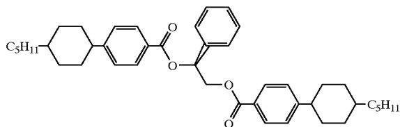
(Chemical 3)
