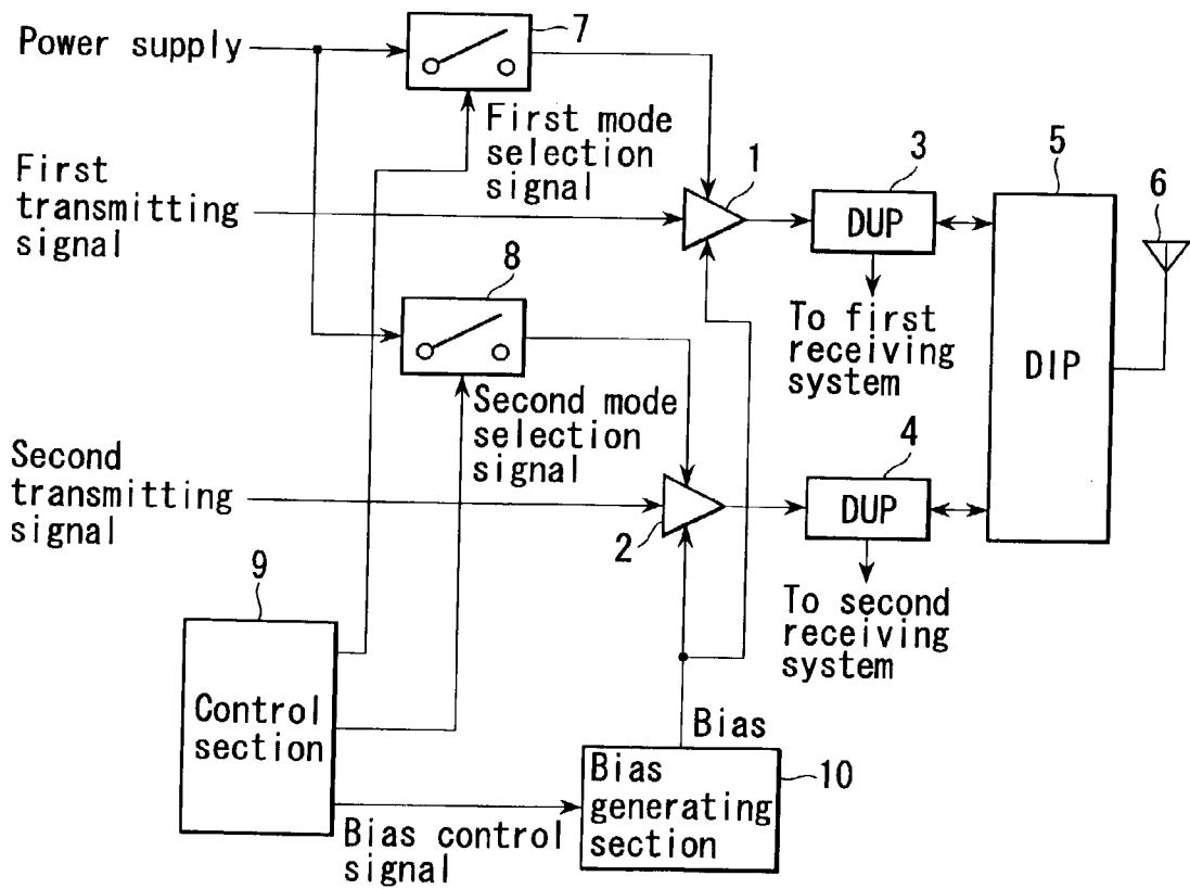
FIG. 4 (PRIOR ART)
