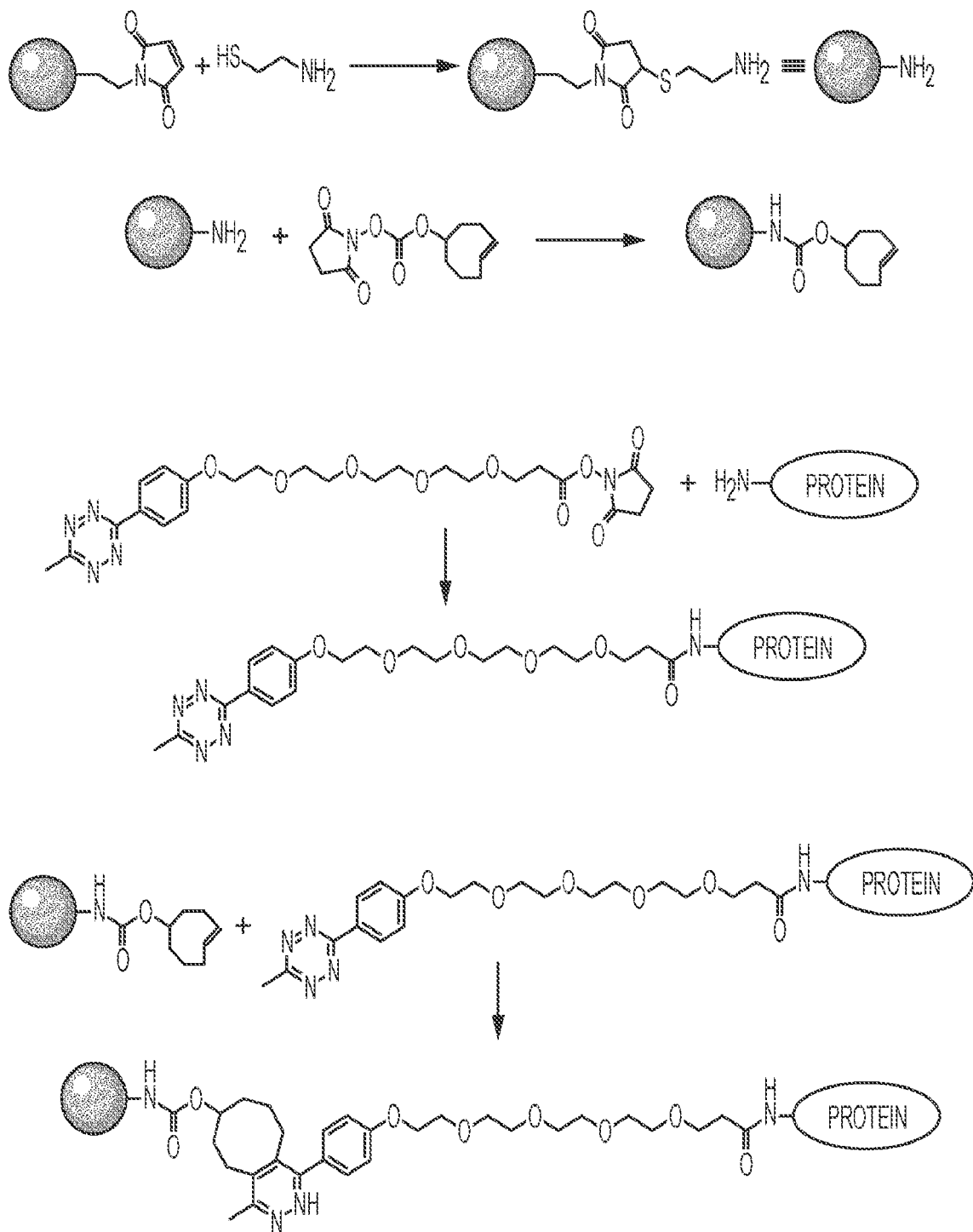
SCHEME 2. ALKENE-TETRAZINE CHEMISTRY
