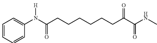
alpha-cetoamide
