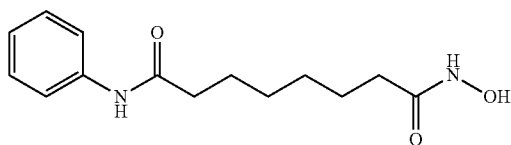
N-hydroxy-N'-phenyl-octanediamide
