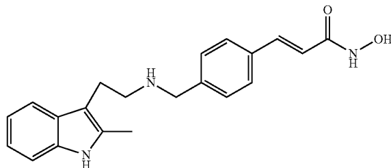
(2E)-N-hydroxy-3-[4-({[2-(2-methyl-1H-indol-3-yl)ethyl]amino}methyl)phenyl]acrylamide
