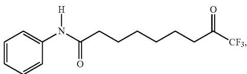
Trifluoromethyl cetone
