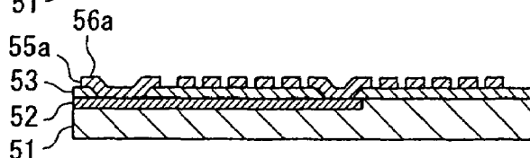
Fig. 15I Prior Art
