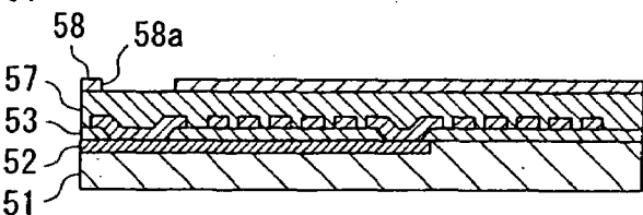
Fig. 15L Prior Art
