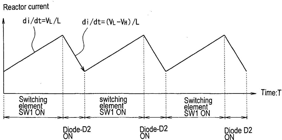
Fig. 8 Prior Art
