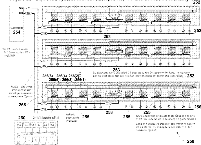
Figure 2c - Improved system with encoded primary CS and decoded secondary CS
