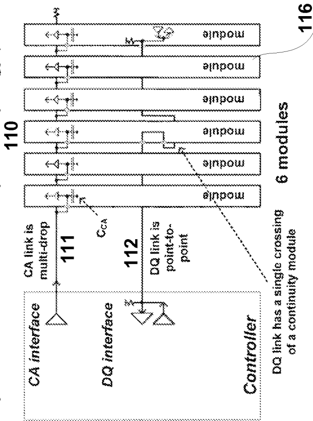
Fig 1e - DQ and CA links — Improved topology (6 module)
