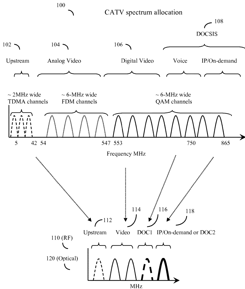
Simplified CATV spectrum diagram
