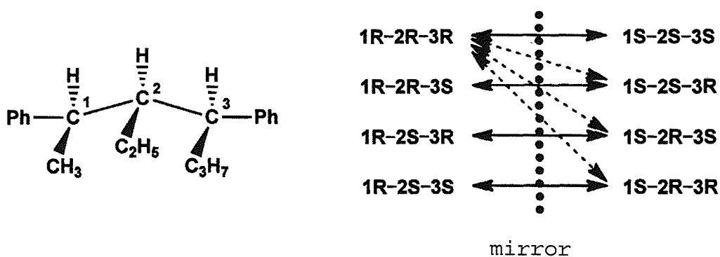
[Formula 7]
