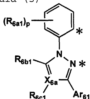
Formula (5)
