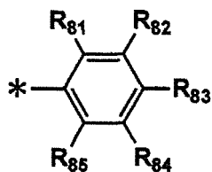
Formula (4)
