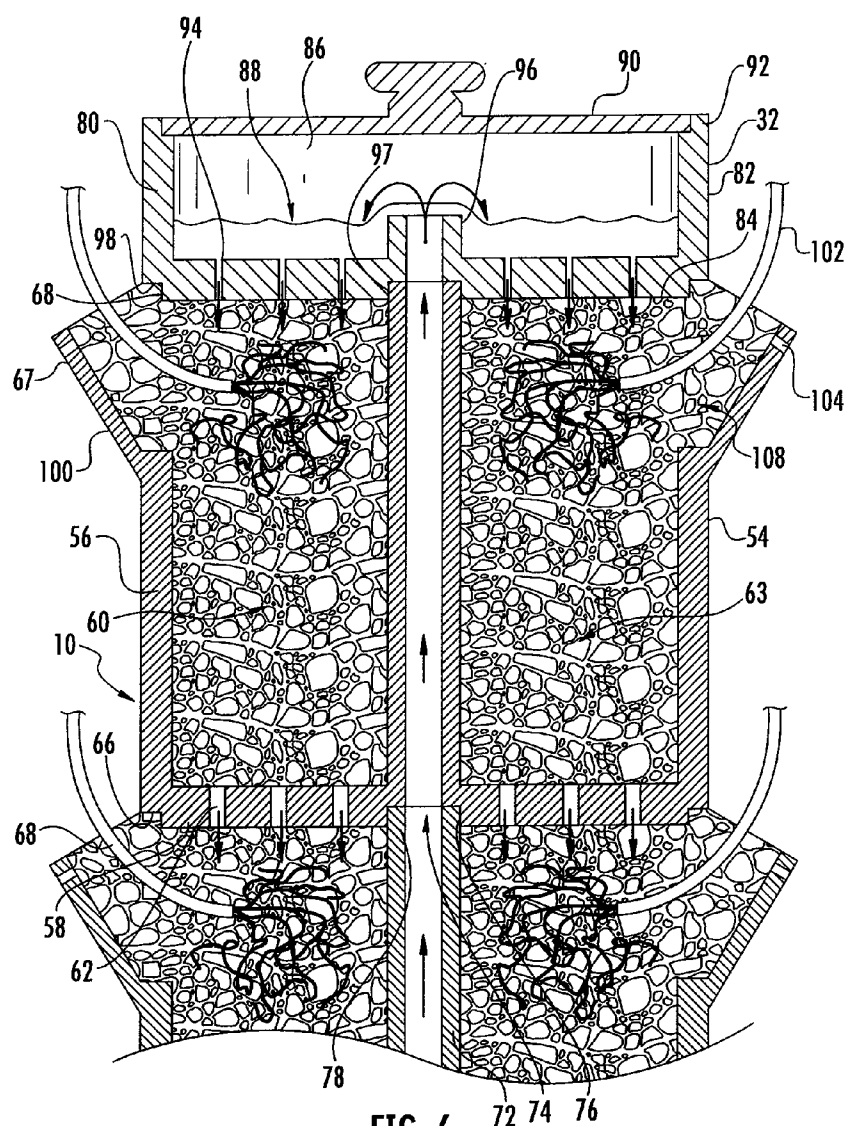
FIG. 6 (PRIOR ART)
