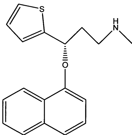
Duloxetine/(S)-Duloxetine
