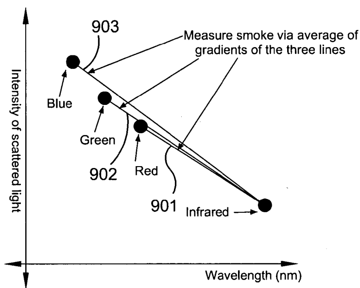
FIGURE 9A Scattering vs Wavelength - average of gradient to IR to measure smoke
