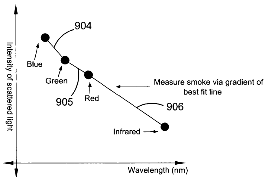
FIGURE 9B Scattering vs Wavelength - average of gradient to measure smoke
