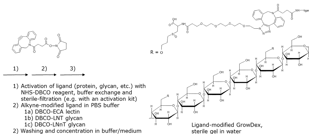
Scheme 2.
