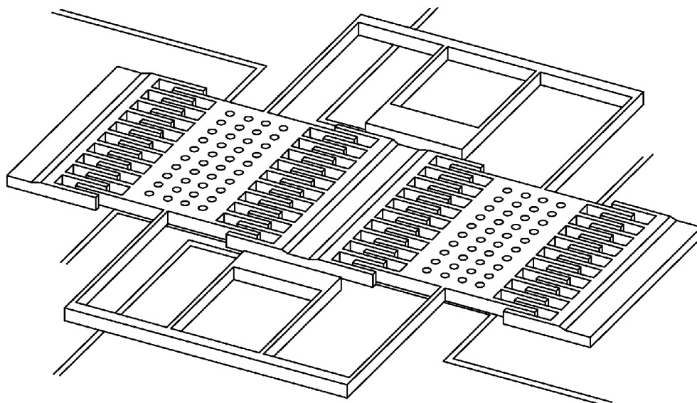
Comb-drive tuning forks MEMS gyroscope
