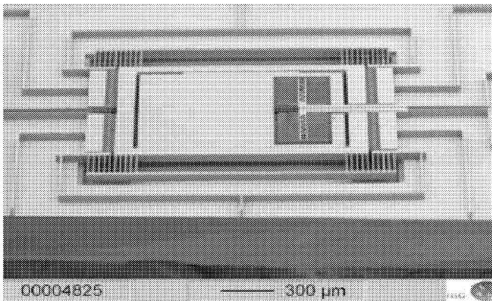
Linear resonator gyroscope, from web-page of HSG-IMIT
