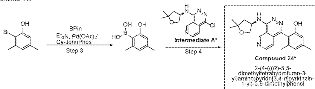
Scheme 9C
