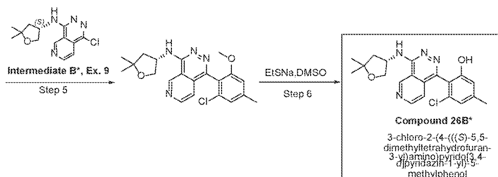
Scheme 11B
