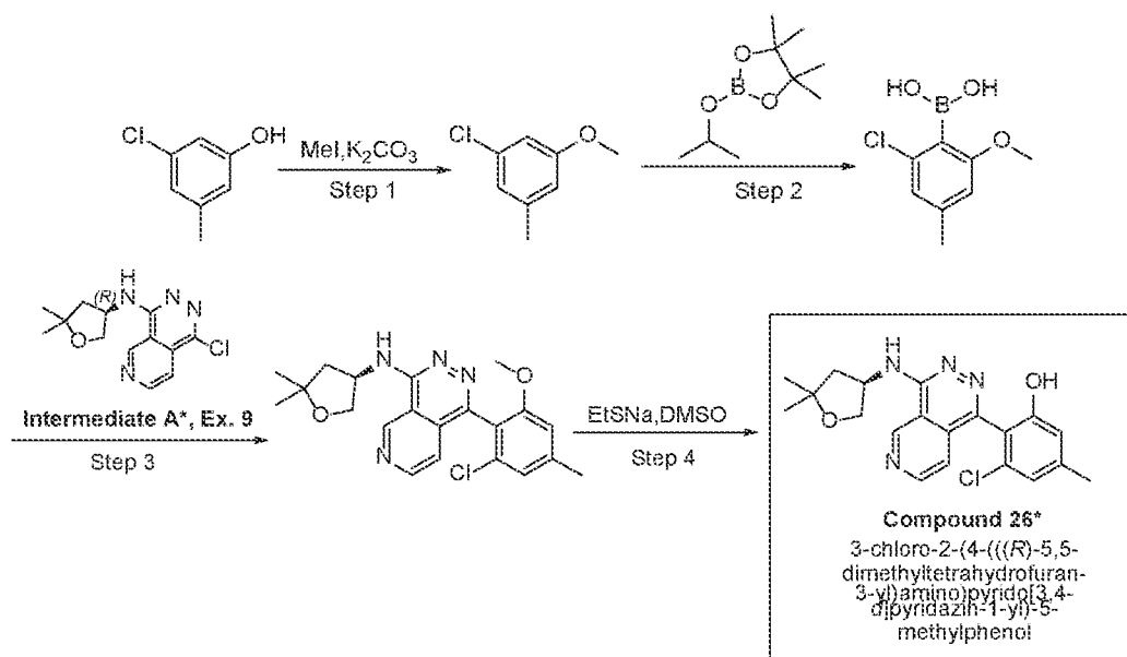
Scheme 11B
