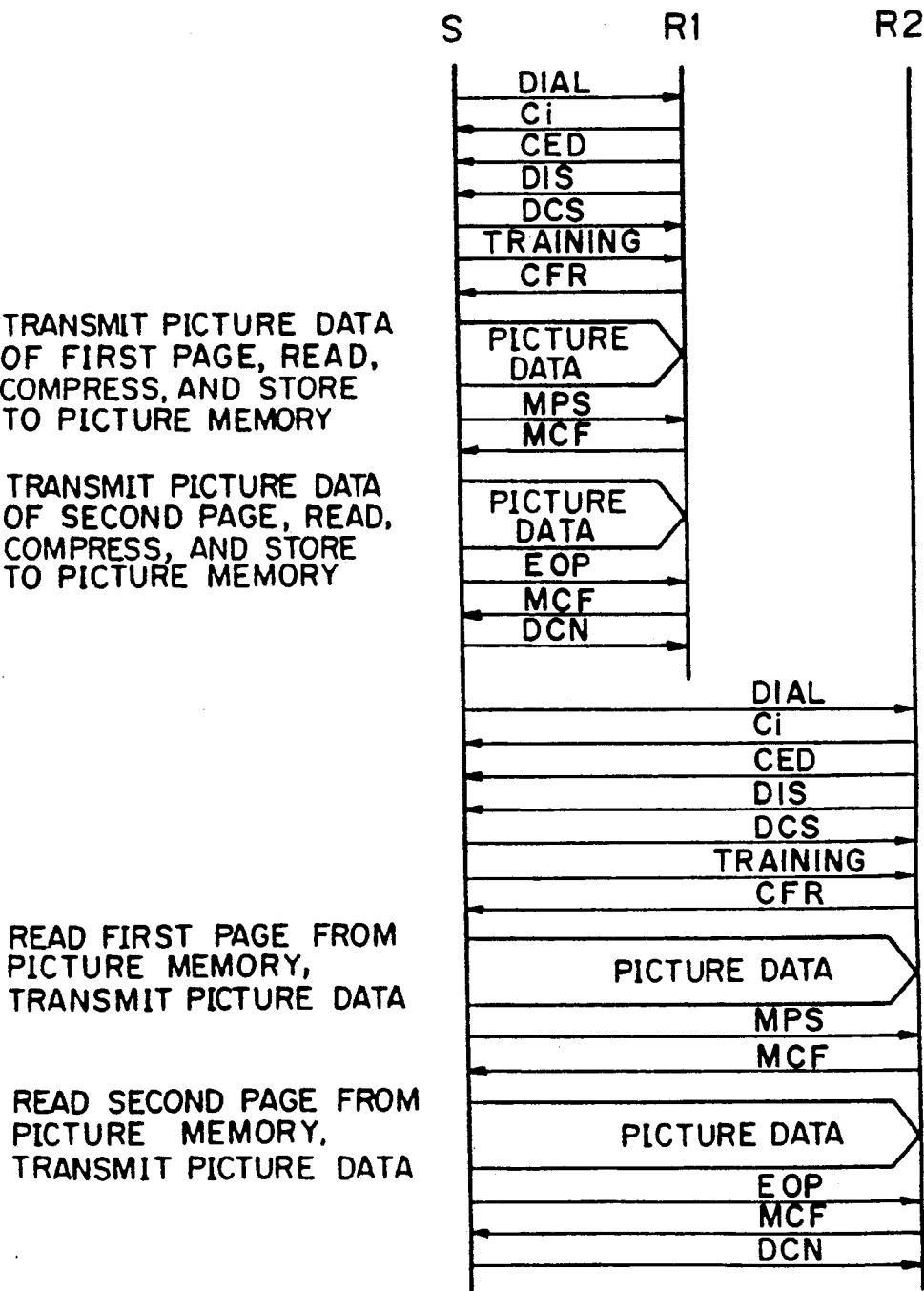
Fig. 4 PRIOR ART
