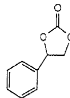
4-phenyl-1,3-dioxolan-2-one
