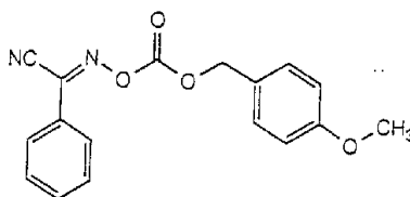
2-(4-methoxybenzyloxycarbonyloxyimino)-2-phenylacetonitrile
