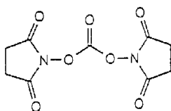
Di(succinimidy) carbonate
