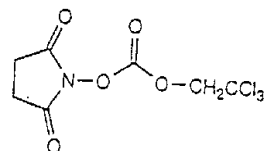
Succinimidyl-2,2,2-trichloroethyl carbonate
