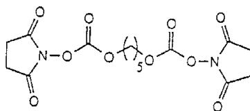
1,5-Bis(succinimidooxycarbonyloxy)pentane
