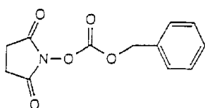
N-(Benzyloxycarbonyloxy)succinimide
