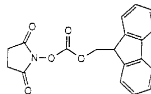
N-(9-Fluorenylmethoxycarbonyloxy)succinimide
