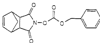
N-Benzyloxycarbonyloxy-5-norbornene-2,3-dicarboximide
