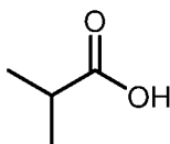
isobutyric acid
