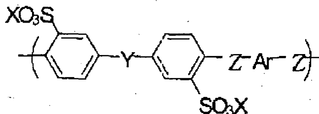
(general formula 14)
