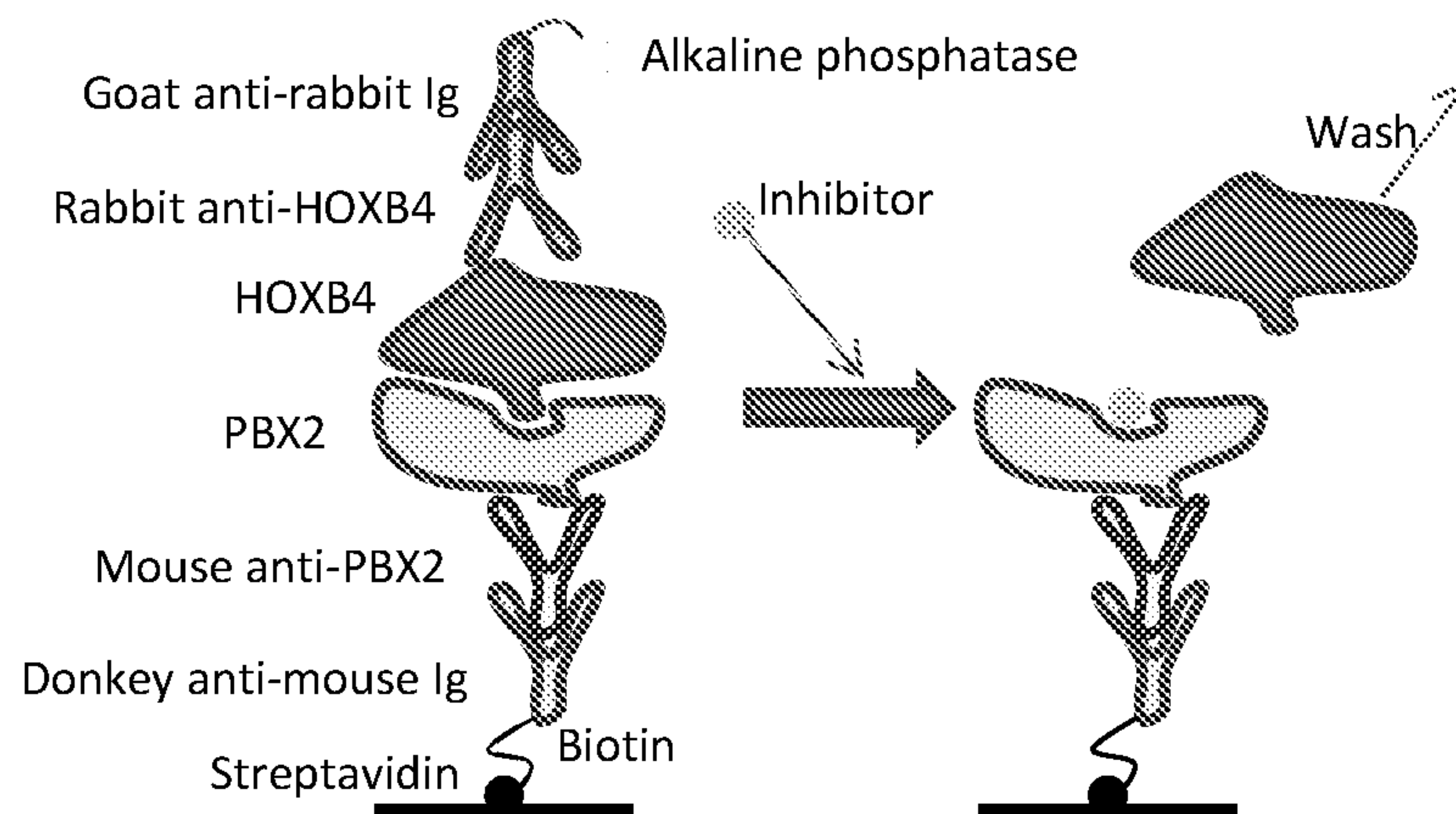
Figure 8: Schematic for HOXB4/PBX2 dimer assay
