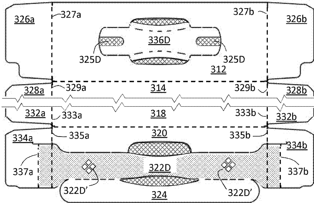
310D FIGURE 28
