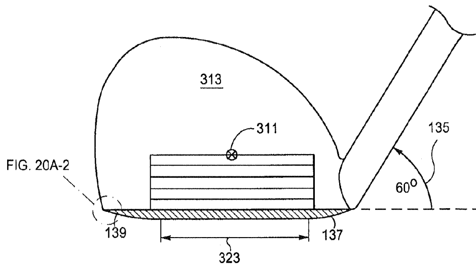
FIG. 20A-1 FRONT VIEW
