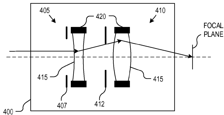
ADAPTIVE ZOOM MODULE (INVERTED TELEPHOTO SETTING – WIDE FOV & LOW MAGNIFICATION)
