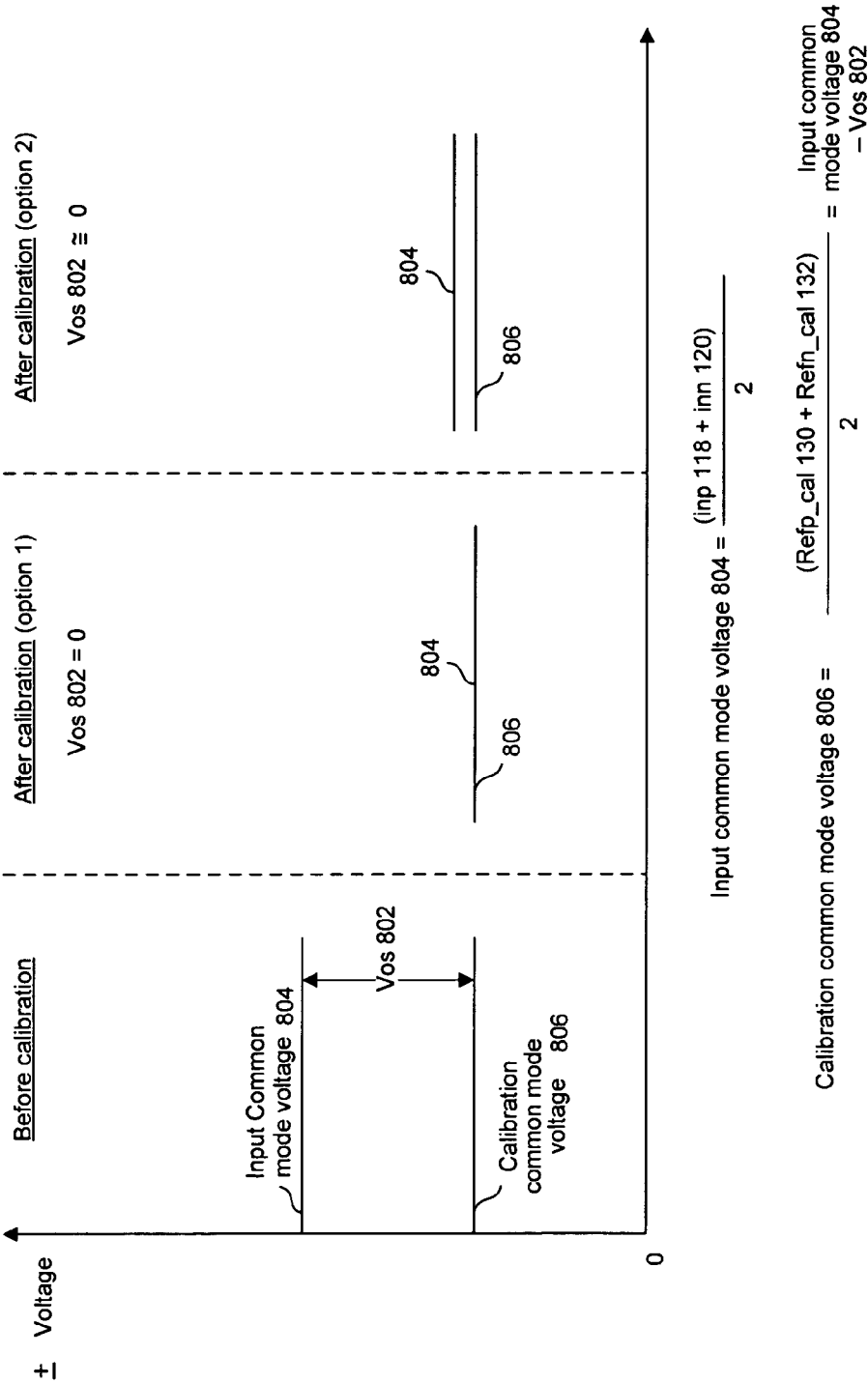
ADC Common Mode Voltage Offset
