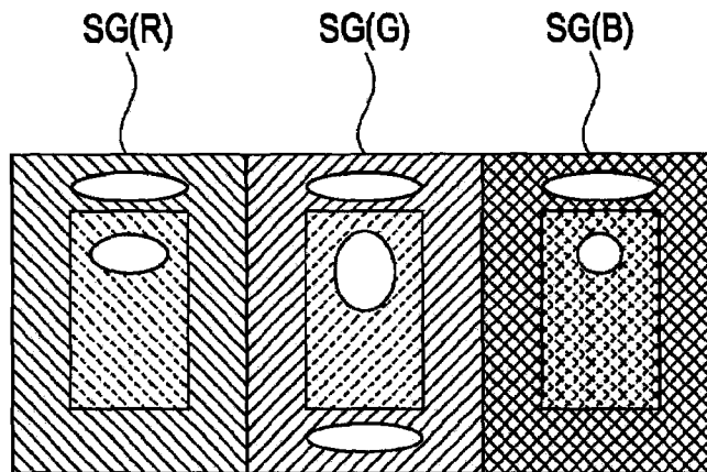
FIG. 8 EXAMPLE OF GENERAL RGB PIXEL ARRANGEMENT STRUCTURE
