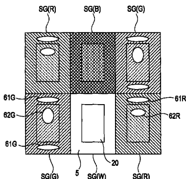
EXAMPLE OF ARRANGEMENT STRUCTURE OF DISPLAY PIXEL
