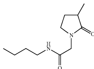
N-n-butyl-(3-methyl-2-oxo-pyrrolidino)-acetamide;
