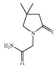
(3,4-dimethyl-2-oxo-pyrrolidino)-acetamide;
