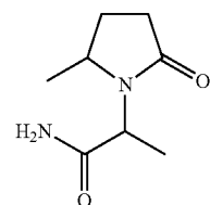
2-(5-methyl-2-oxo-pyrrolidino)-propionamide;
