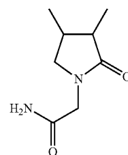
(3,4-dimethyl-2-oxo-pyrrolidino)-acetamide;
