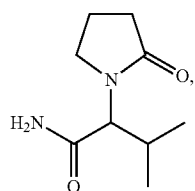
2-(2-oxo-pyrrolidino)-3-methyl-butyramide;
