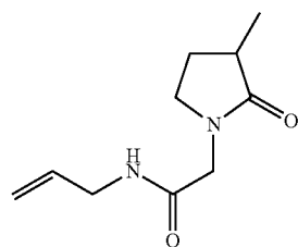
N-allyl-(3-methyl-2-oxo-pyrrolidino)-acetamide;
