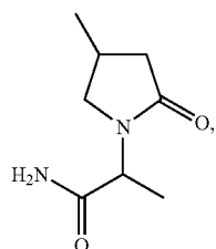
2-(4-methyl-2-oxo-pyrrolidino)-propionamide;
