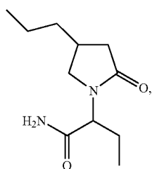
2-(4-propyl-2-oxo-pyrrolidino)-butyramide (also known as "brivaracetam");
