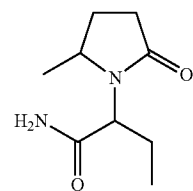
2-(5-methyl-2-oxo-pyrrolidino)-butyramide;
