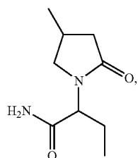
2-(4-methyl-2-oxo-pyrrolidino)-butyramide;
