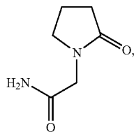
2-(2-oxo-pyrrolidino)-acetamide (also known as "piracetam");
