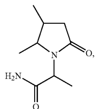
2-(4,5-dimethyl-2-oxo-pyrrolidino)-propionamide;
