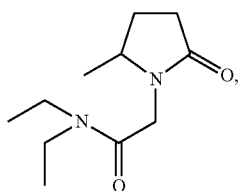
(5-methyl-2-oxo-pyrrolidino)-N,N-diethylacetamide;
