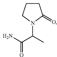
2-(2-oxo-pyrrolidino)-propionamide;
