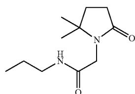
N-n-propyl-(5,5-dimethyl-2-oxo-pyrrolidino)-acetamide;
