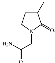
(3-methyl-2-oxo-pyrrolidino)-acetamide;
