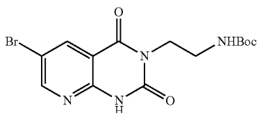
Tert-butyl (2-(6-bromo-2-oxo-1,4-dihydropyrido[2,3-d]pyrimidin-3(2H)-yl)ethyl)carbamate (E-24)
