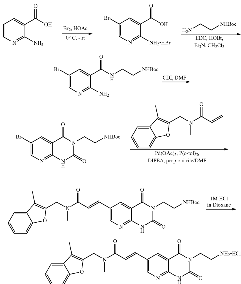
Scheme 3. Synthesis of Naphthyridinone Analogs E22-E26 (see Table 5 in Example 4)
