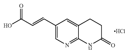
(E)-3-(7-oxo-5,6,7,8-tetrahydro-1,8-naphthyridin-3-yl)acrylic acid hydrochloride (E-28)
