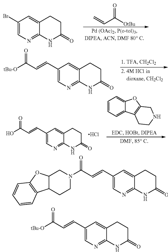
Scheme 4. Synthesis of Analogs with Reduced Rotatable Bonds E27-E29 (see Table 5 in Example 4)
