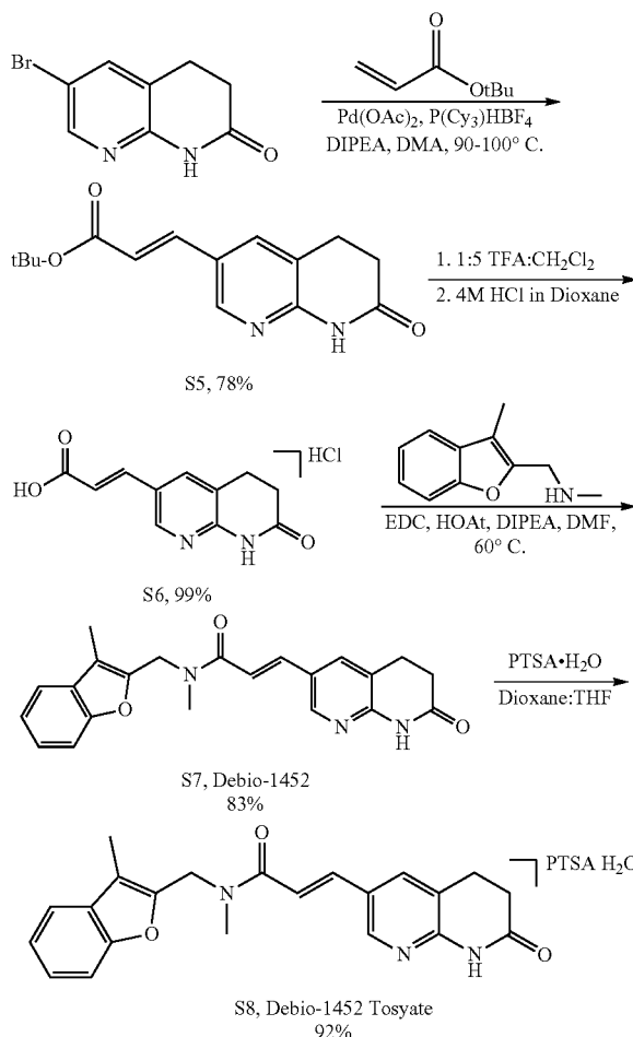
Scheme C. Synthesis of Debio-1452 Tosylate.
