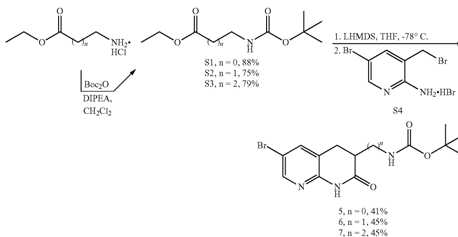
Scheme B. Synthesis of Naphthyridinone Presursors and Debio-1452 Amine Containing Analogues.
