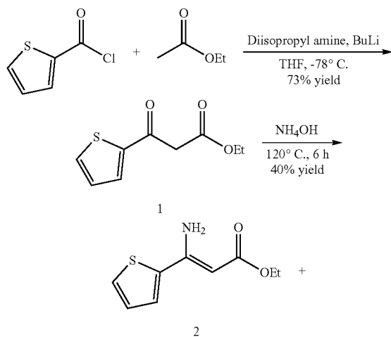
Scheme 6. Synthesis of Fragment 4.
