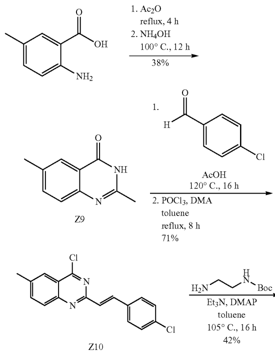
Scheme 5. Synthesis of quinazoline derivatives.
