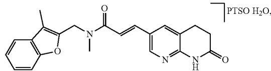
Debio-1452 Tosylate
