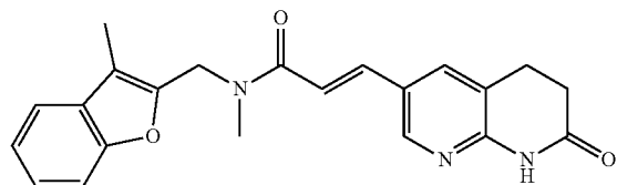
Debio-1452
