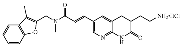
(E)-3-(6-(aminoethyl)-7-oxo-5,6,7,8-tetrahydro-1,8-naphthyridin-3-yl)-N-methyl-N-((3-methylbenzofuran-2-yl)methyl)acrylamide hydrochloride (E-17)
