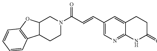
(E)-6-(3-oxo-3-(3,4,4a,9a-tetrahydrobenzofuro[2,3-c]pyridin-2(1H)-yl)prop-1-en-1-yl)-3,4-dihydro-1,8-naphthyridin-2(1H)-one (E-29)
