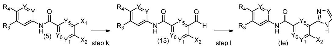
Reaction Scheme VI
