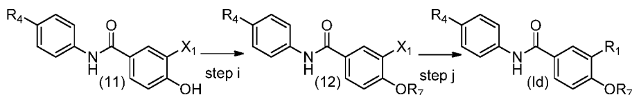
Reaction Scheme V:
