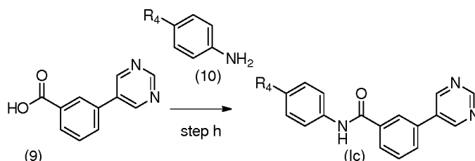
Reaction Scheme IV:
