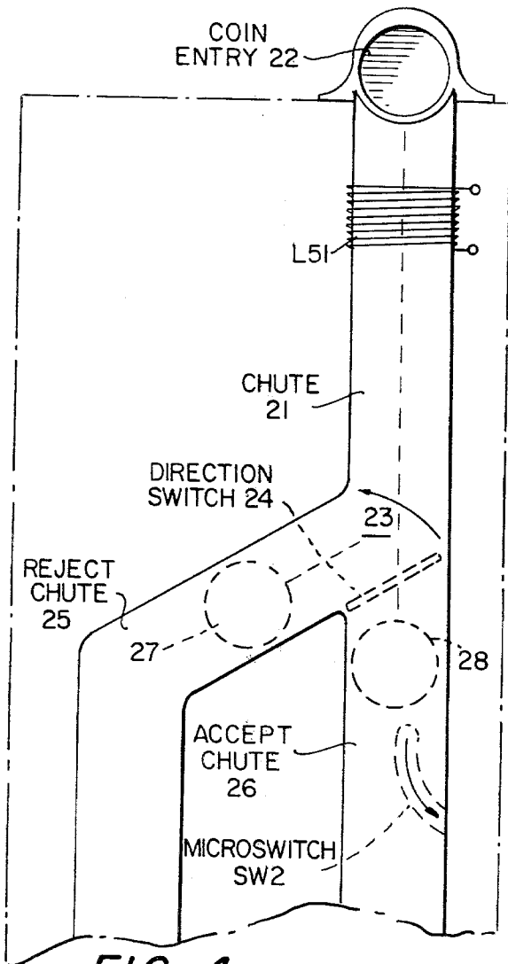
FIG. 4 PRIOR ART
