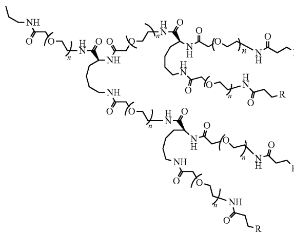
Et-G3-R
