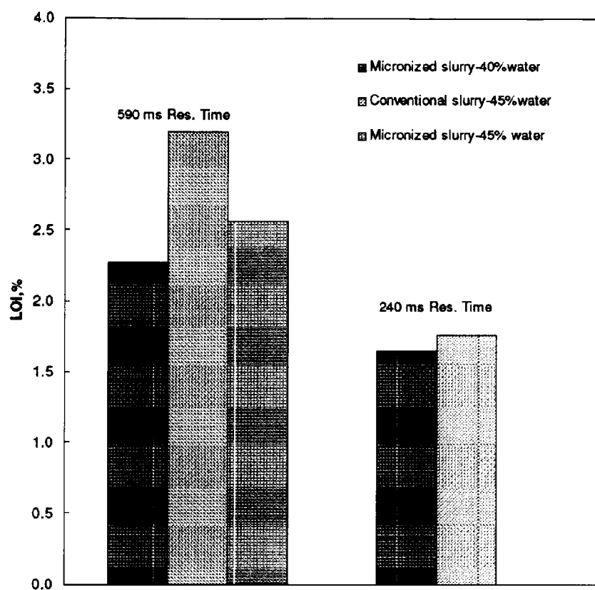
Comparison of Loss on Ignition (LOI).
