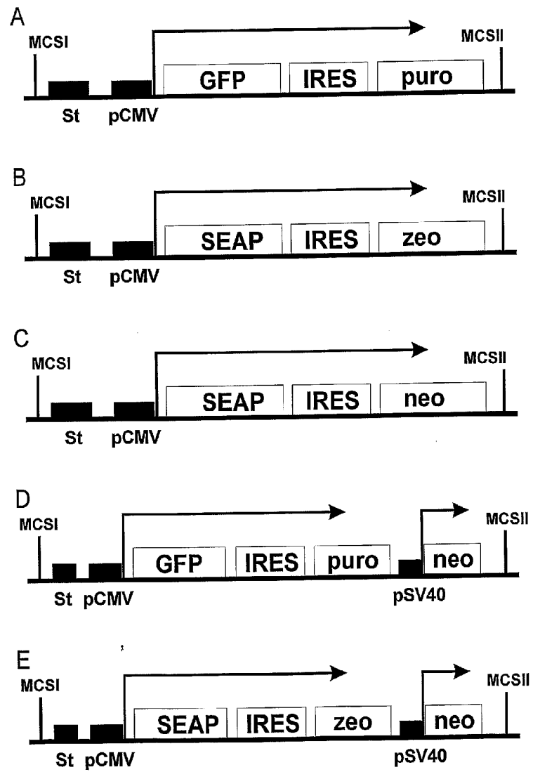
FIG 5 The PP family of plasmids
