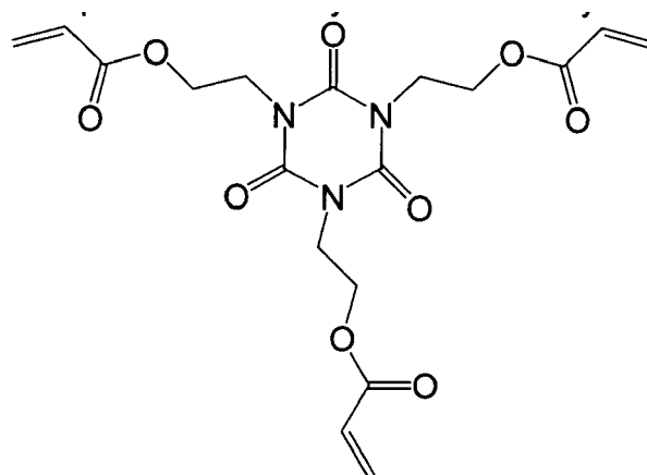
Compound B-7: urethane acrylate of MDL / pentaerythritol triacrylate
