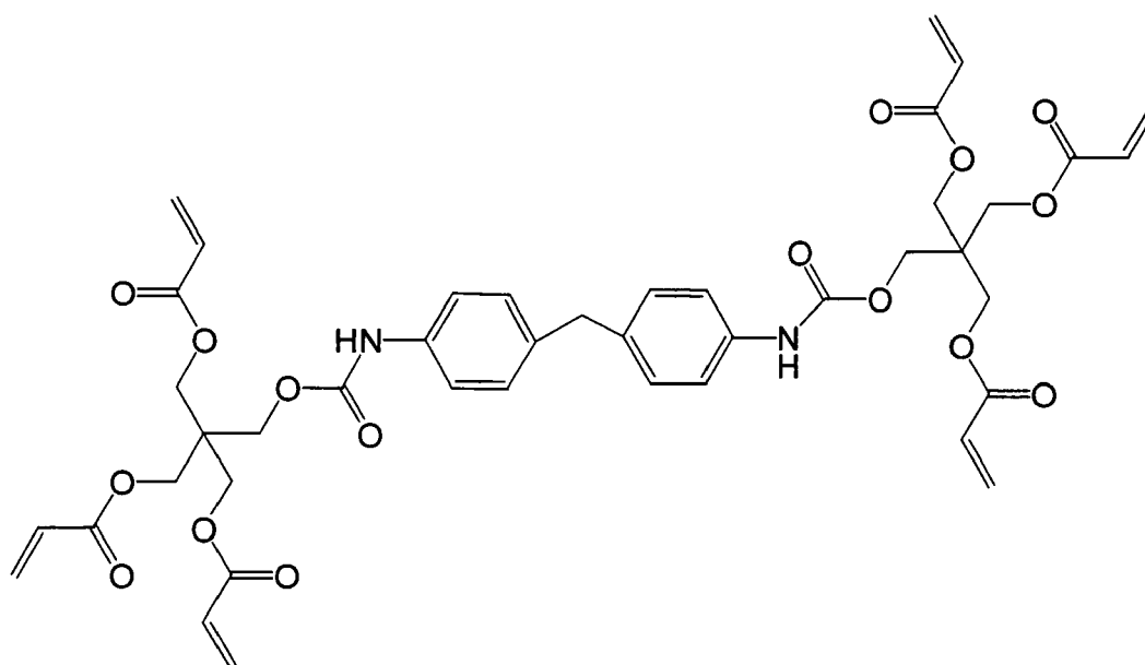
[0112] Compound B-8: urethane acrylate of norbornene diisocyanate / pentaerythritol triacrylate
