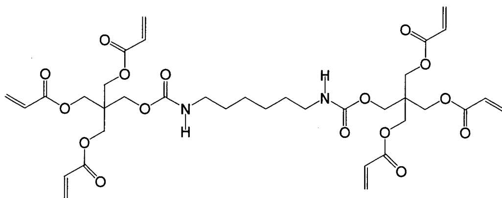
Compound B-5: polyester acrylate of adipic acid / pentaerythritol triacrylate
