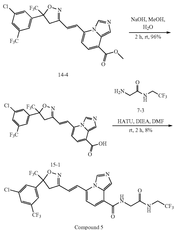
Scheme 15
