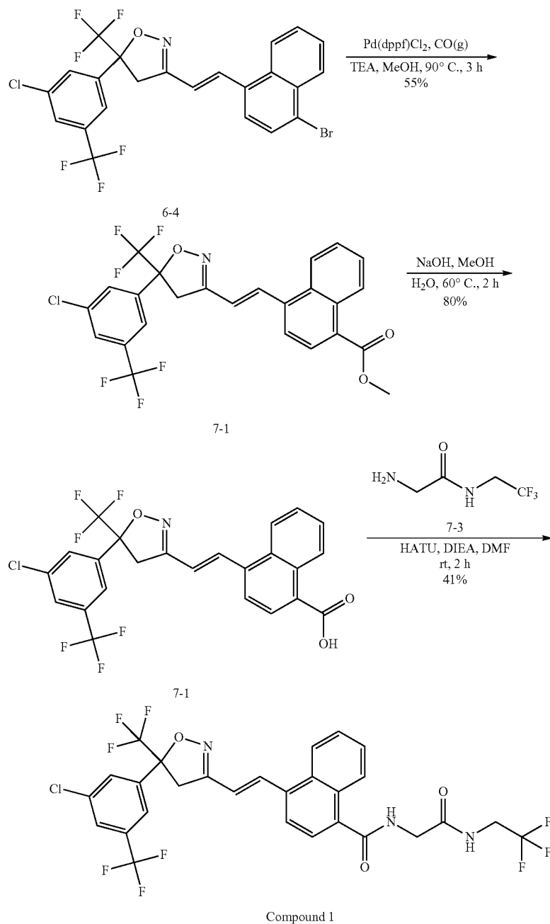
Scheme 7
