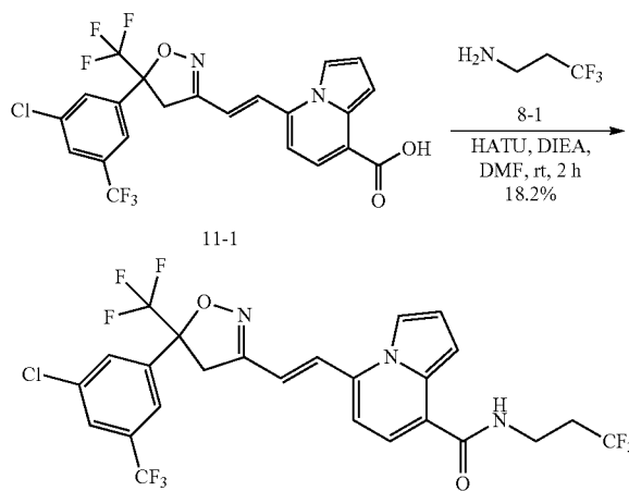
Compound 4
