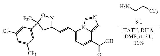
Scheme 16
