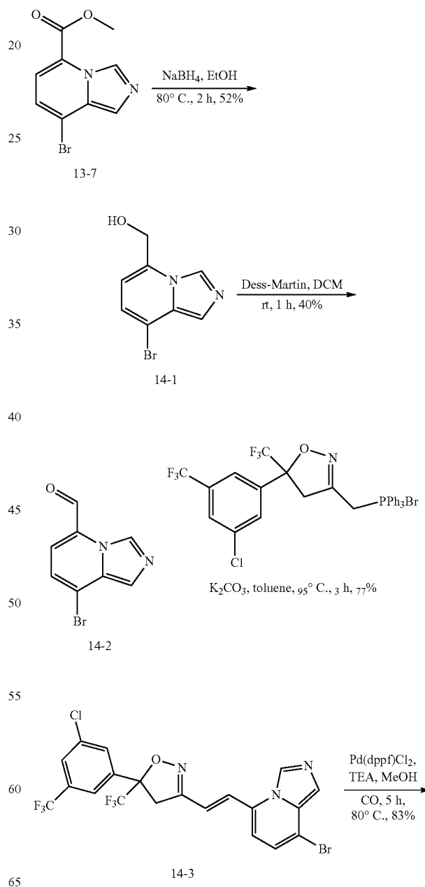
Scheme 14
