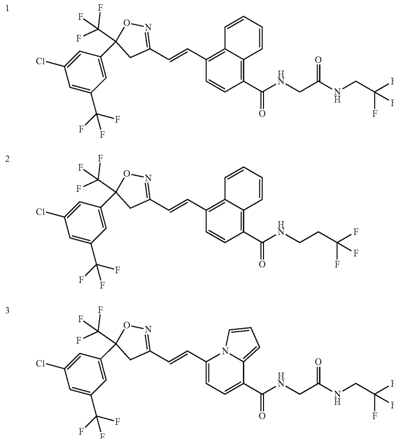
Compound # Structure
