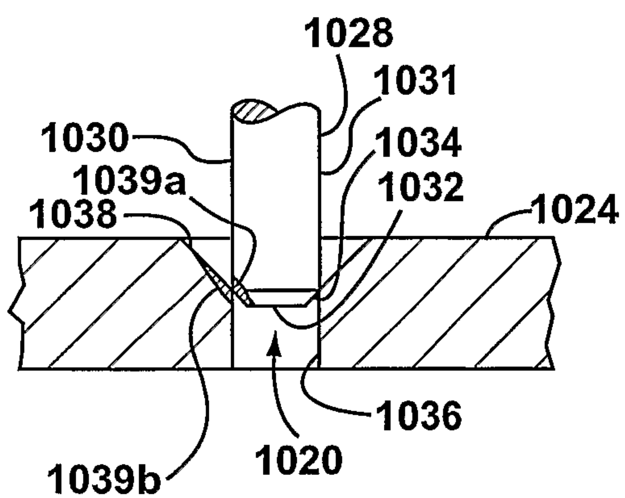
FIG. 2c (PRIOR ART)
