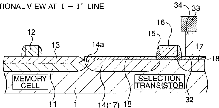
SECTIONAL VIEW CORRESPONDING TO I — I' LINE
