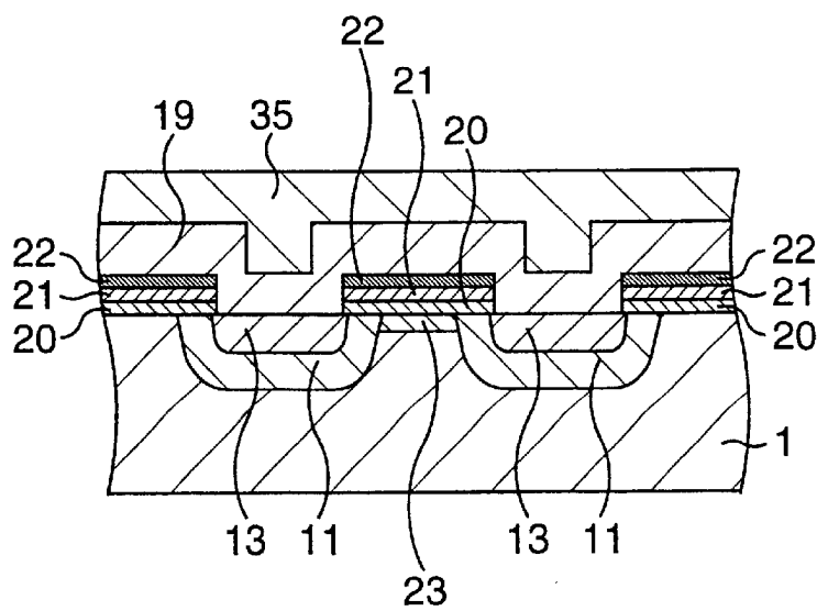
FIG.3 SECTIONAL VIEW CORRESPONDING TO III – III' LINE
