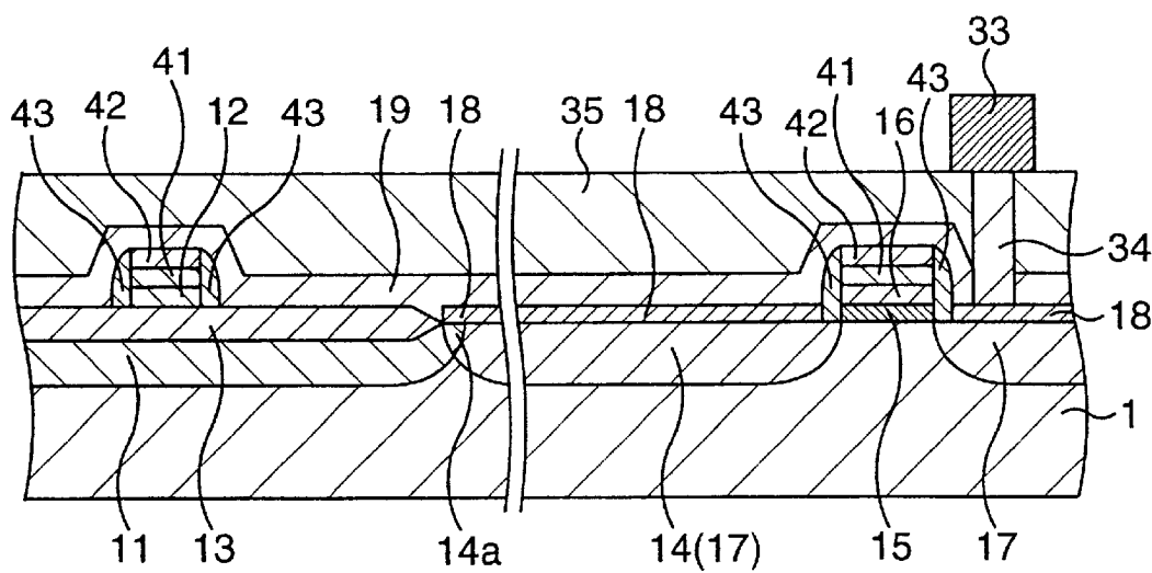
FIG.3 SECTIONAL VIEW CORRESPONDING TO I – I' LINE
