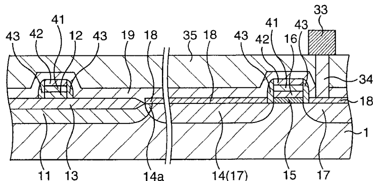
SECTIONAL VIEW CORRESPONDING TO I — I' LINE
