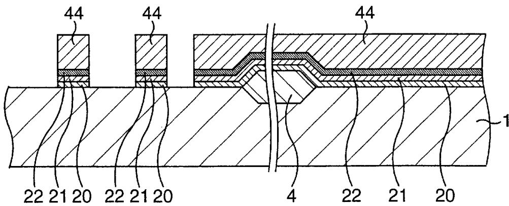
FIG.9 SECTIONAL VIEW CORRESPONDING TO I – I' LINE
