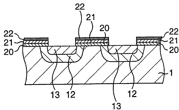
FIG.3 SECTIONAL VIEW CORRESPONDING TO III – III' LINE
