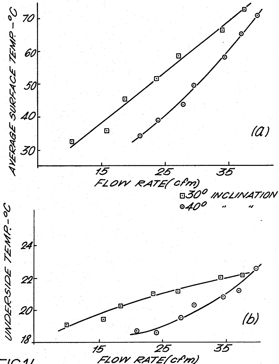
FIG.14. VARIATION OF FLOW RATE WITH SURFACE TEMP. AND UNDERSIDE TEMP. (TABLES 9 & 10)
