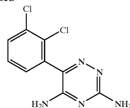
Lamotrigine 1 15.6% yield
