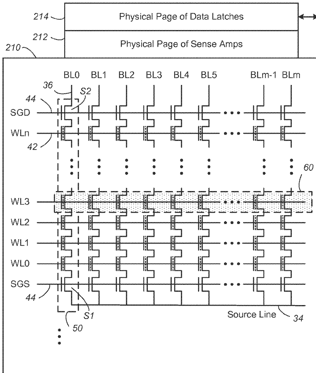
FIG. 5 (PRIOR ART)
