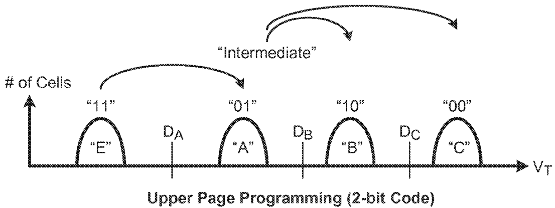
FIG. 7C (PRIOR ART)
