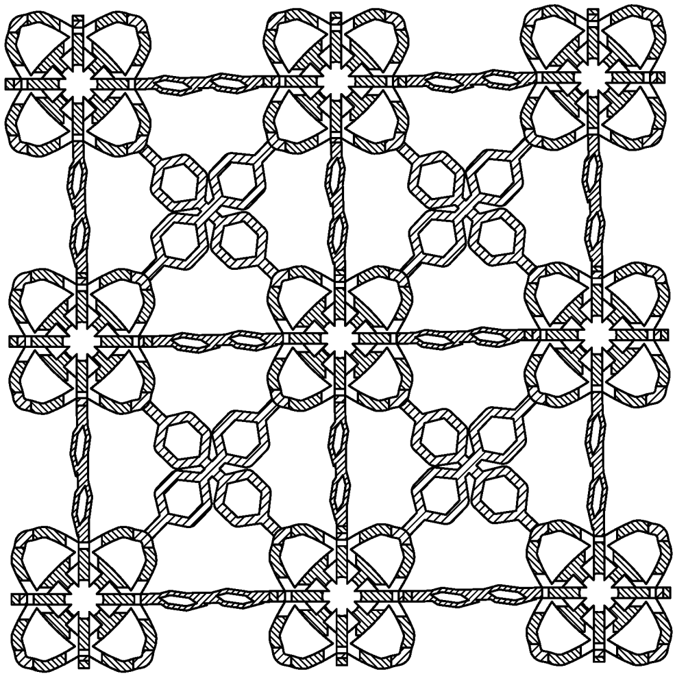
UiO-67 STRUCTURE
