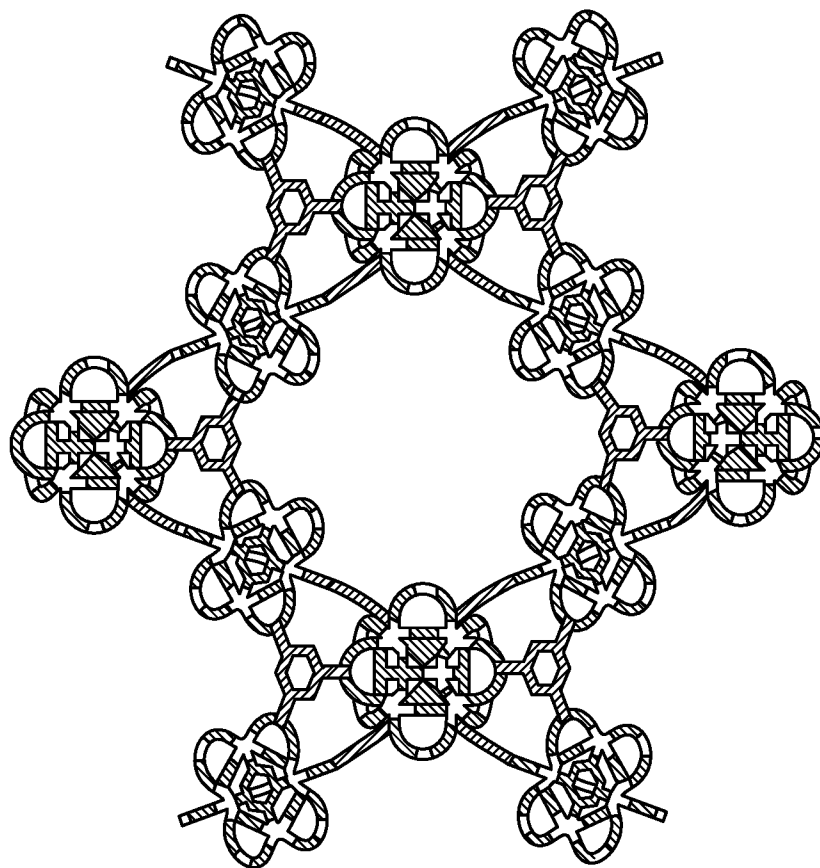
MOF-808 STRUCTURE
