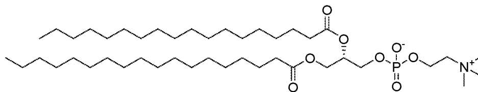
distearoyl phosphatidylcholine (DSPC)
