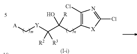
Scheme 7 Process G
