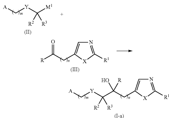
Scheme 1 Process A
