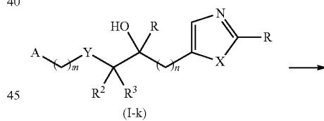
Scheme 9 Process I
