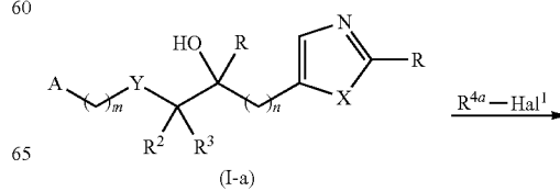
Scheme 10 Process J
