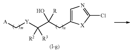
Scheme 6 Process F
