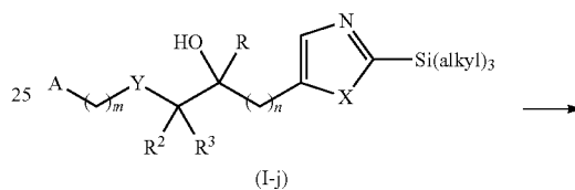
Scheme 8 Process H
