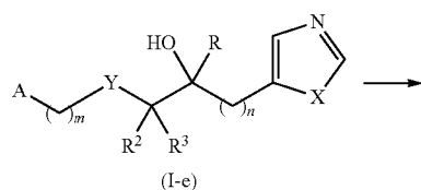
Scheme 5 Process E
