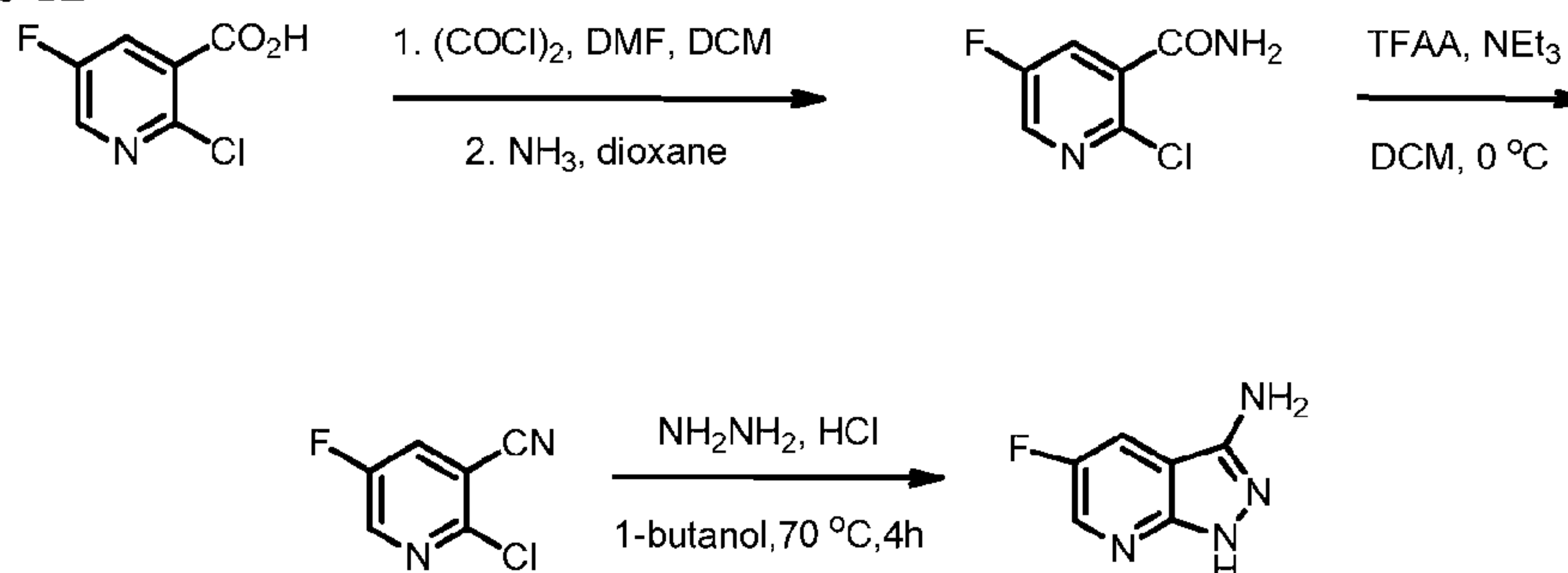
Scheme 12
