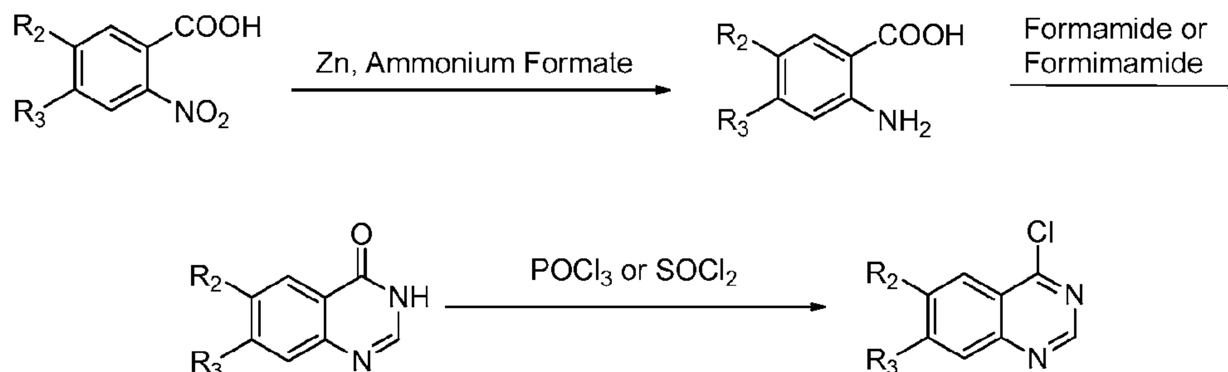
Scheme 1
