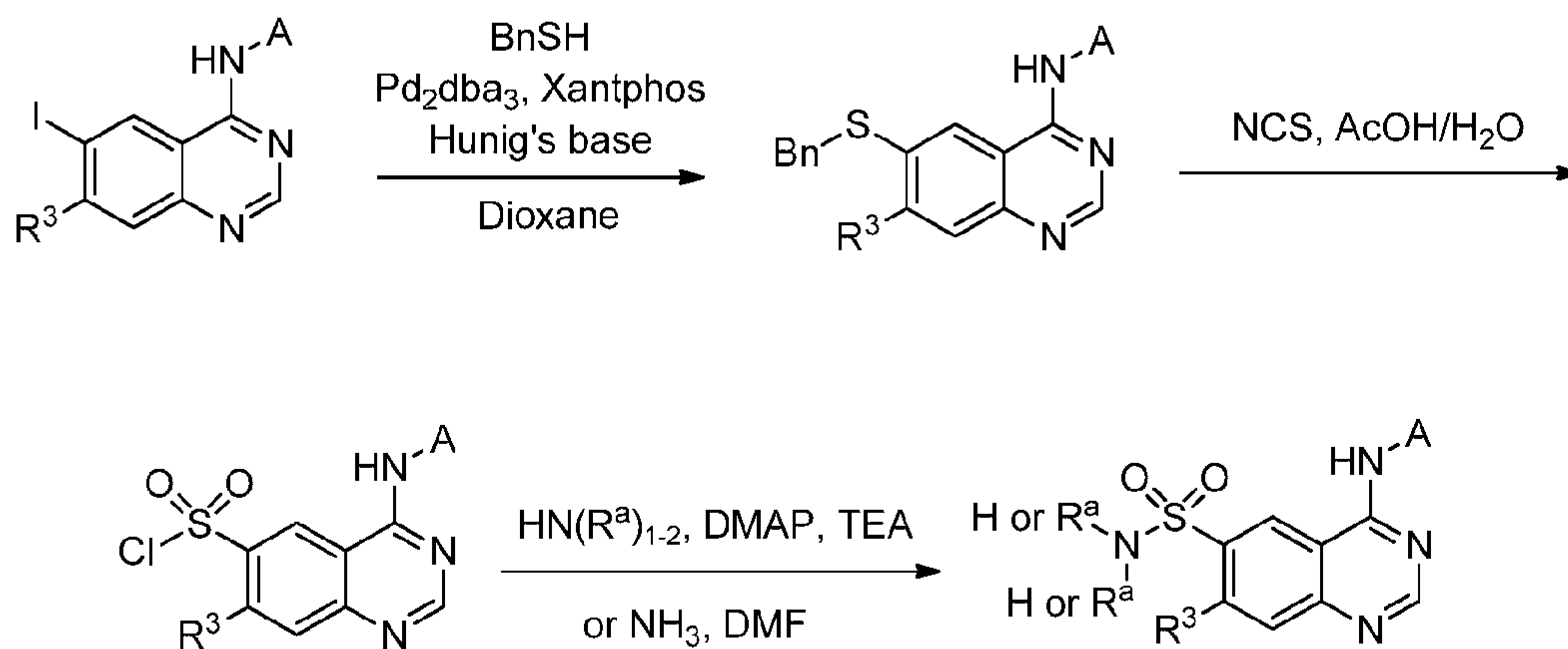
Scheme 19
