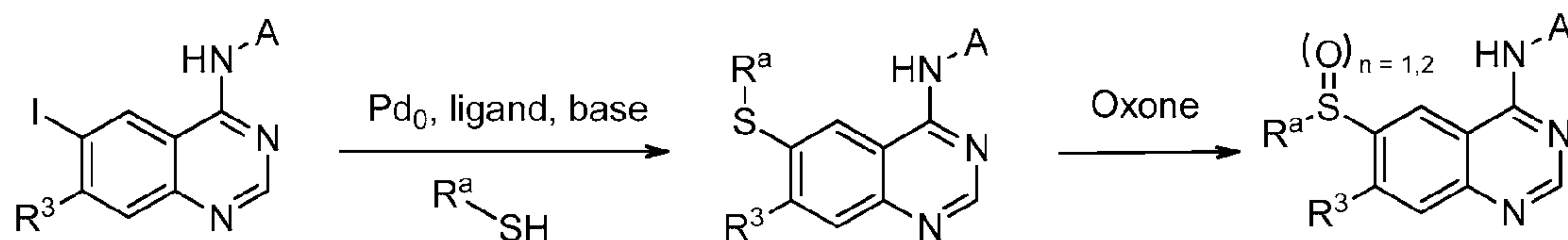
10 Scheme 3
