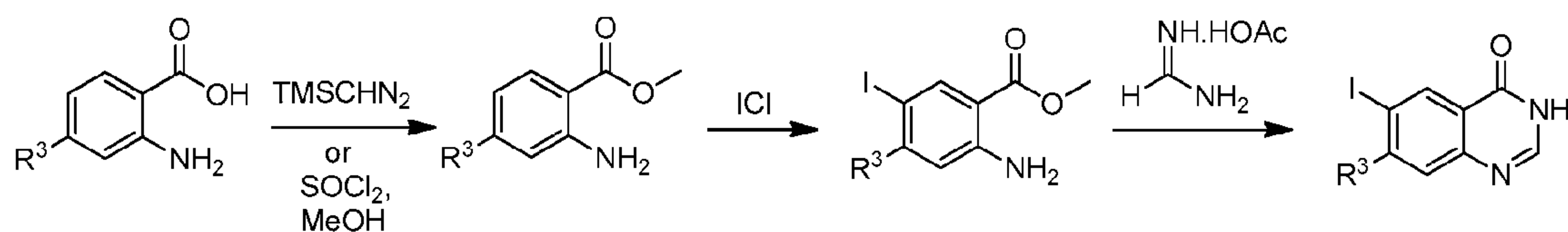
Scheme 2
