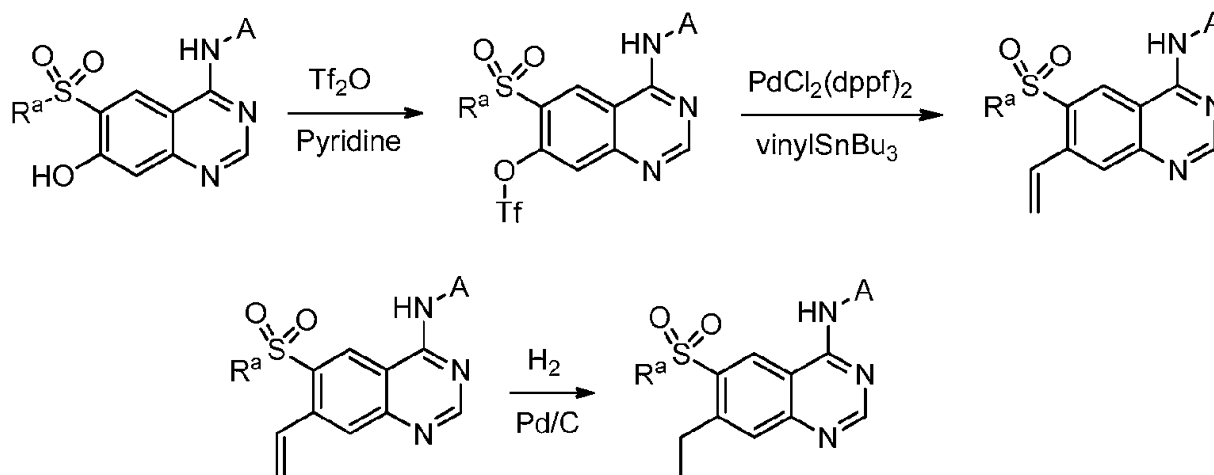
Scheme 10
