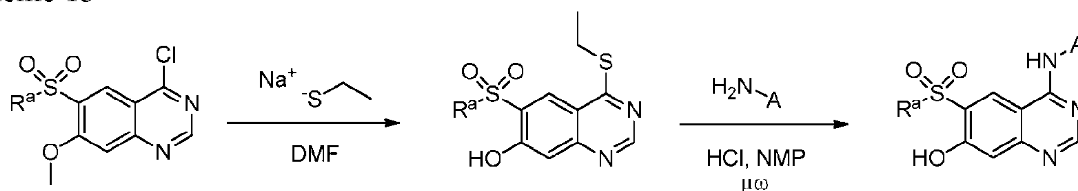
Scheme 15
