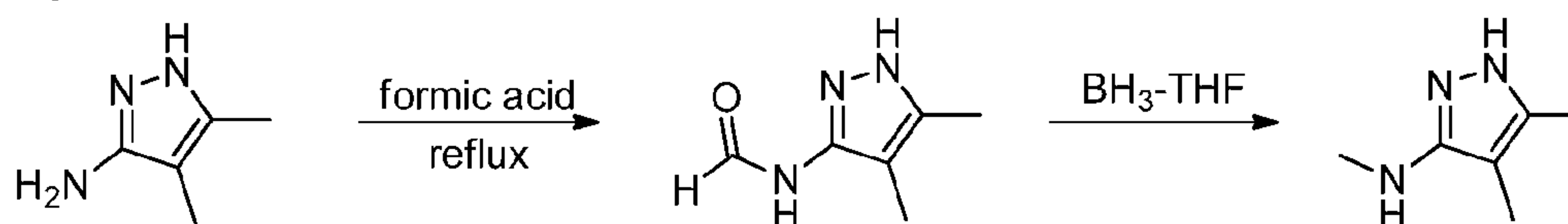
Scheme 14
