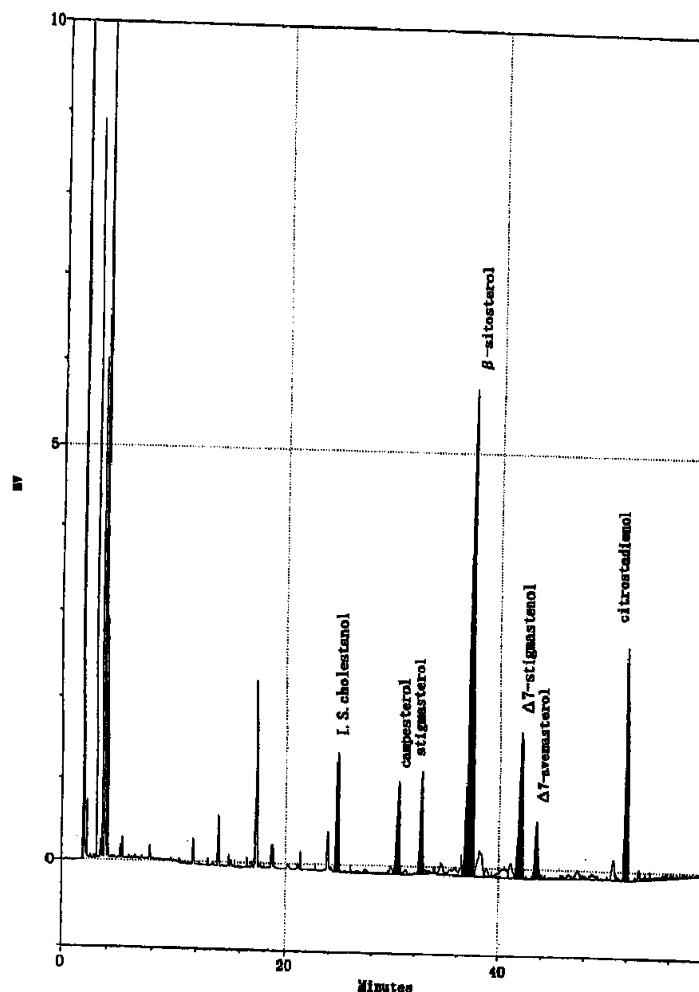
Chromatogram
