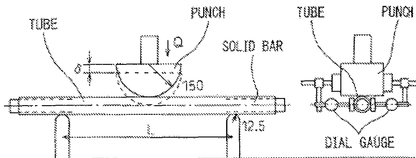
FIG. 4 (Prior Art)
