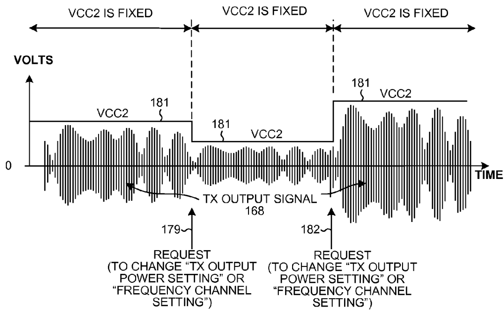
ADAPTIVE AVERAGE POWER TRACKING
