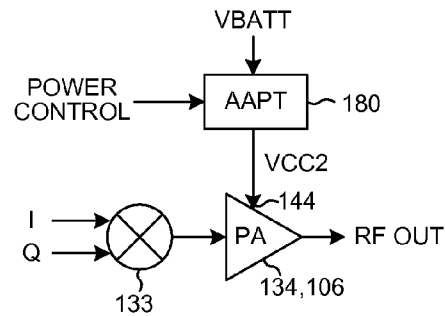
ADAPTIVE AVERAGE POWER TRACKING
