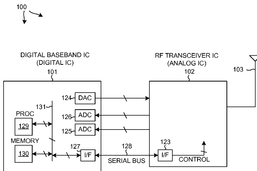
MOBILE COMMUNICATION DEVICE
