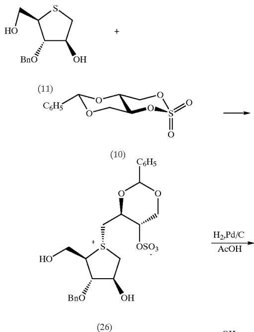
Scheme 10 Synthesis of Salacinol (1)
