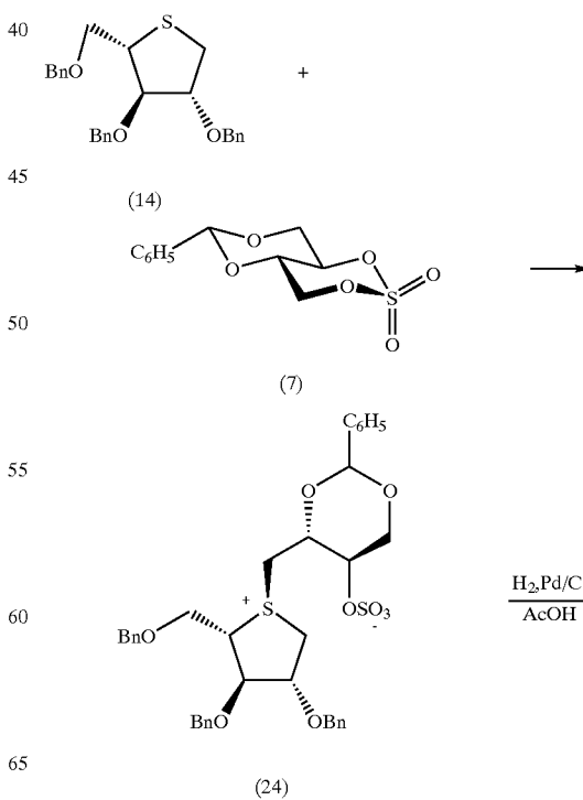
Scheme 9 Synthesis of compound (25)
