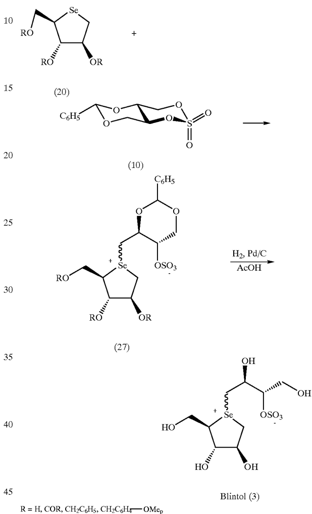
Scheme 11 Synthesis of Blintol (3)
