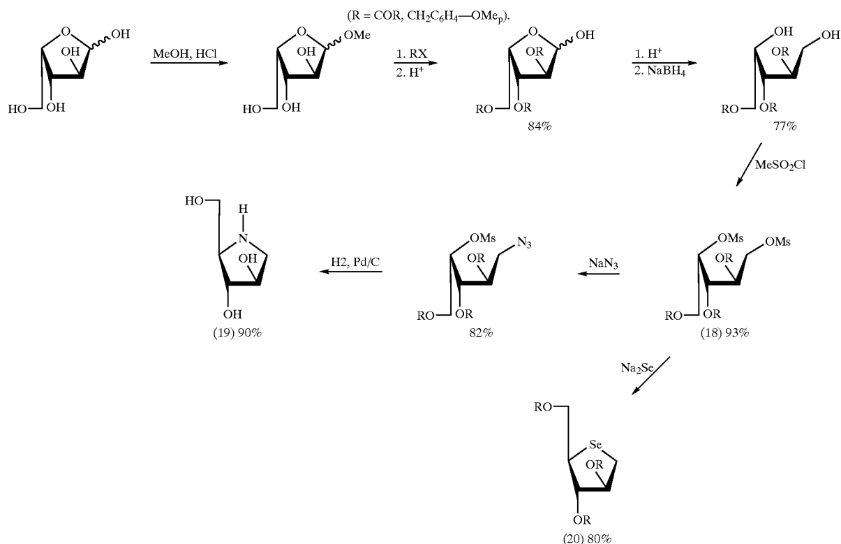
Scheme 6(a). Synthesis of compounds (19) and (20)
