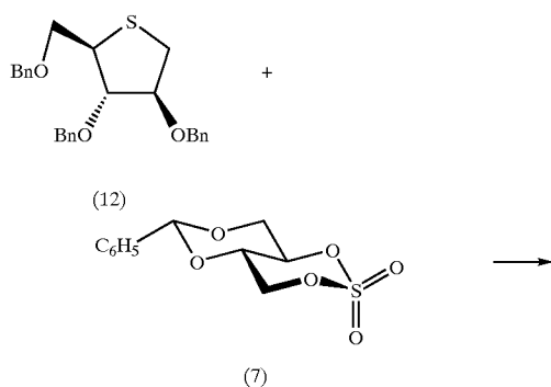
Scheme 8 Synthesis of compound (23)
