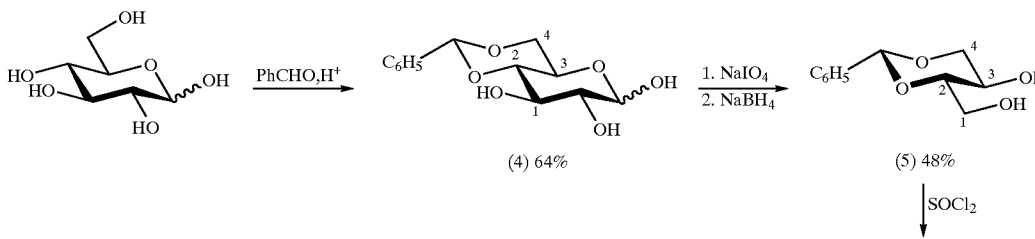
Scheme 2. Synthesis of the cyclic sulfate (7)
