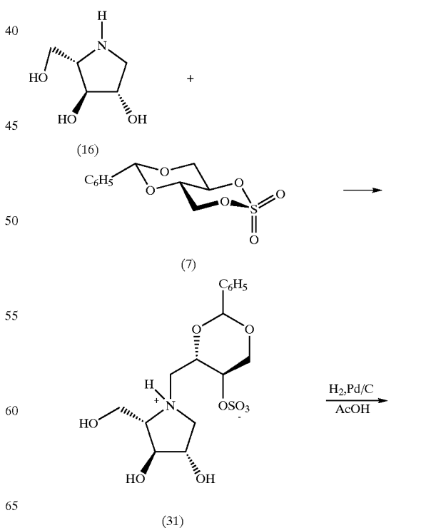
Scheme 14 Synthesis of compound (32)
