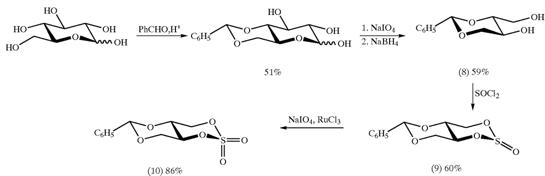
Scheme 3. Synthesis of the cyclic sulfate (10)
