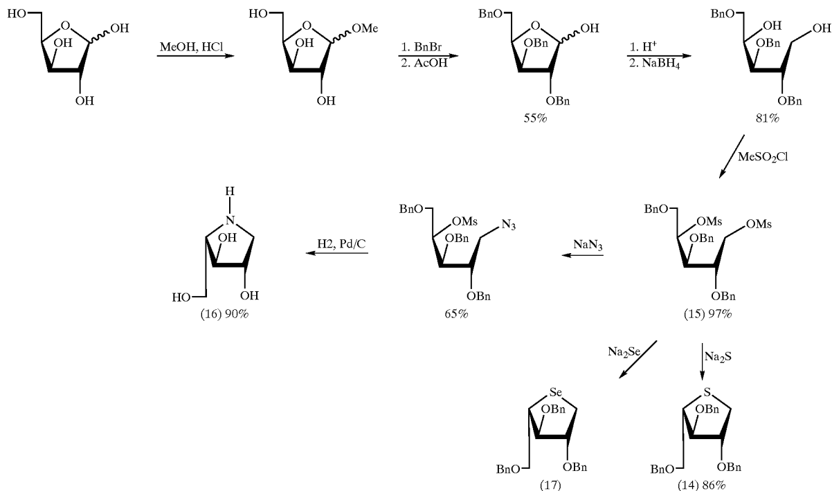
Scheme 5. Synthesis of compounds (14)-(17)
