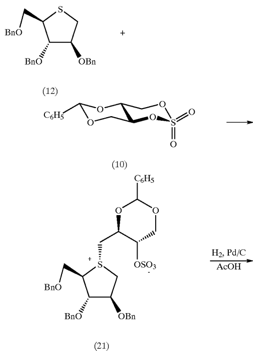
Scheme 7 Synthesis of Salacinol (1)
