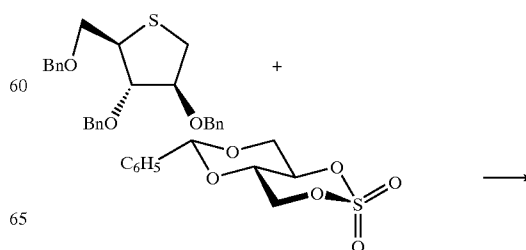
Scheme 8
