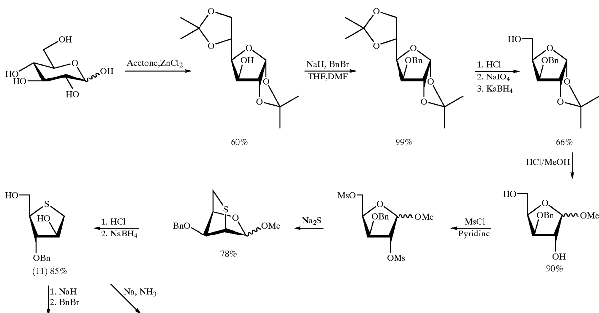
Scheme 4. Synthesis of compounds (11)-(13)
