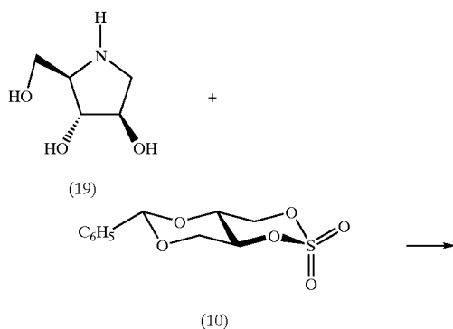
Scheme 13 Synthesis of Ghavamiol (2)
