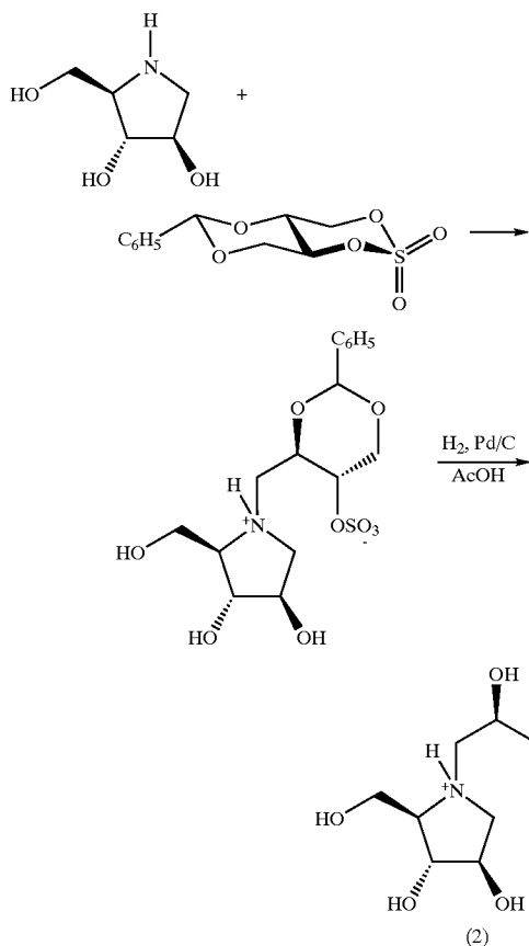
Scheme 13
