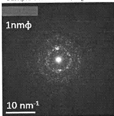
FIG. 9B Sample A3: 130°C, O 2 =10%
