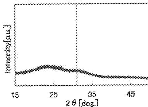
FIG. 9A Sample A3: 130°C, O 2 =10%
